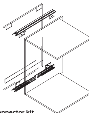
Side panel connector kit 700-604
